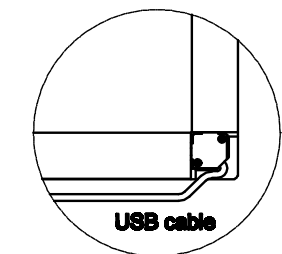
Unilateral cross-section 10:1
