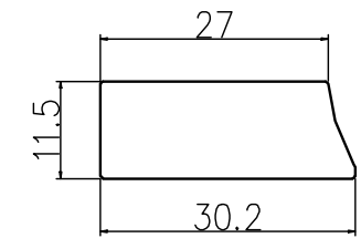
Unilateral cross-section 10:1
