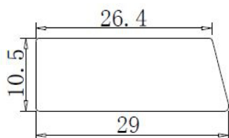
Unilateral cross-section 10:1
